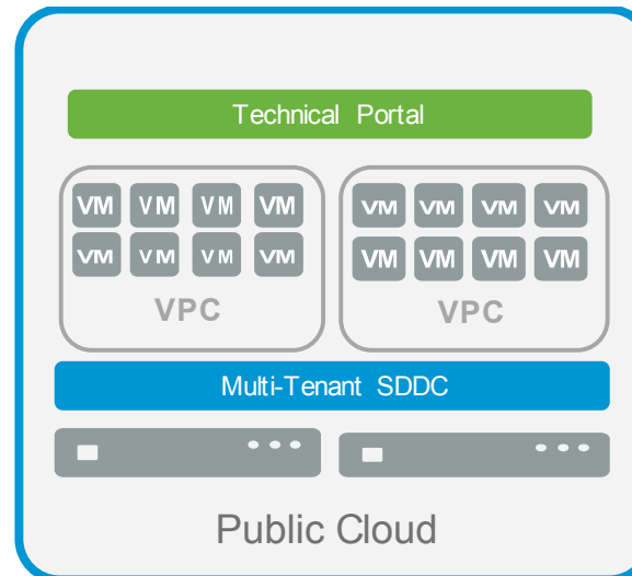
vCloud Director
